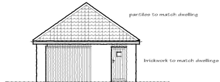
WEST ELEVATION
